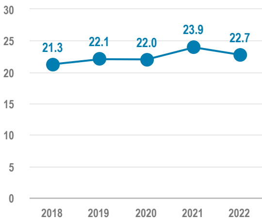
ENERGY INTENSITY (2) GIGAJOULES CONSUMED PER TON OF CRUDE STEEL PRODUCED
